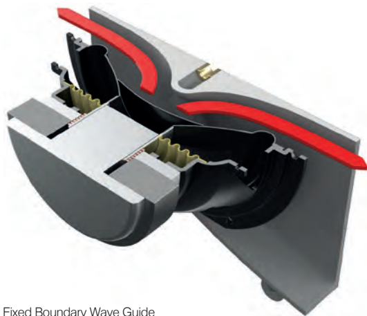
Fixed Boundary Wave Guide
